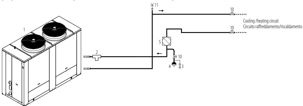
Heat pump with SI+PS/PSI/PD/PDI set-up
