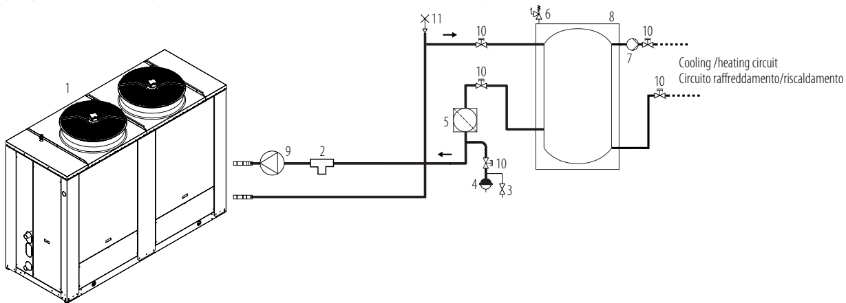
Heat pump with standard set-up
